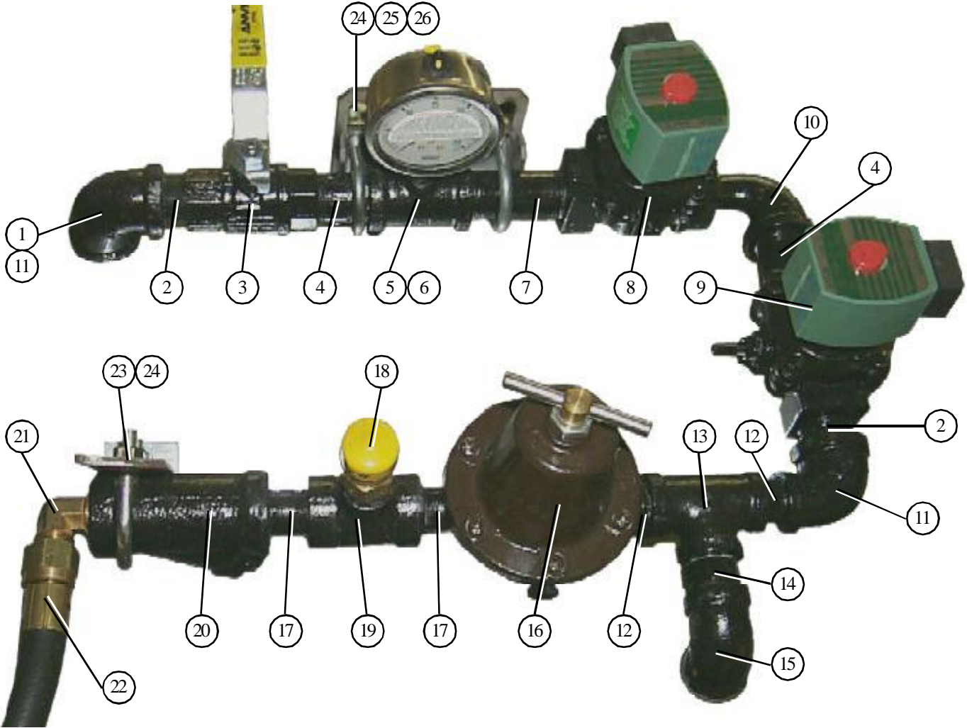
26" & 28" Fan heater LP pipe train assembly.
